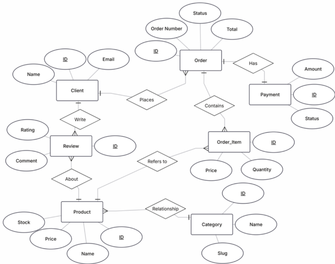
Figure 27: Entity Relationship Diagram (ERD) of the E-Commerce System
