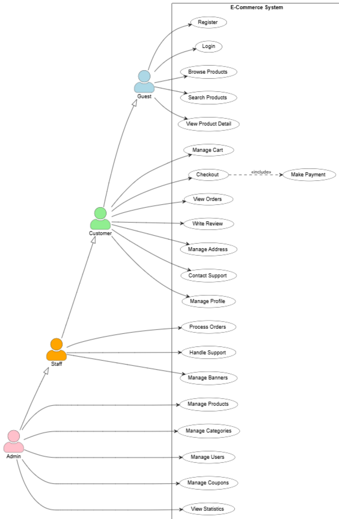
Figure 11: Use case Diagram
